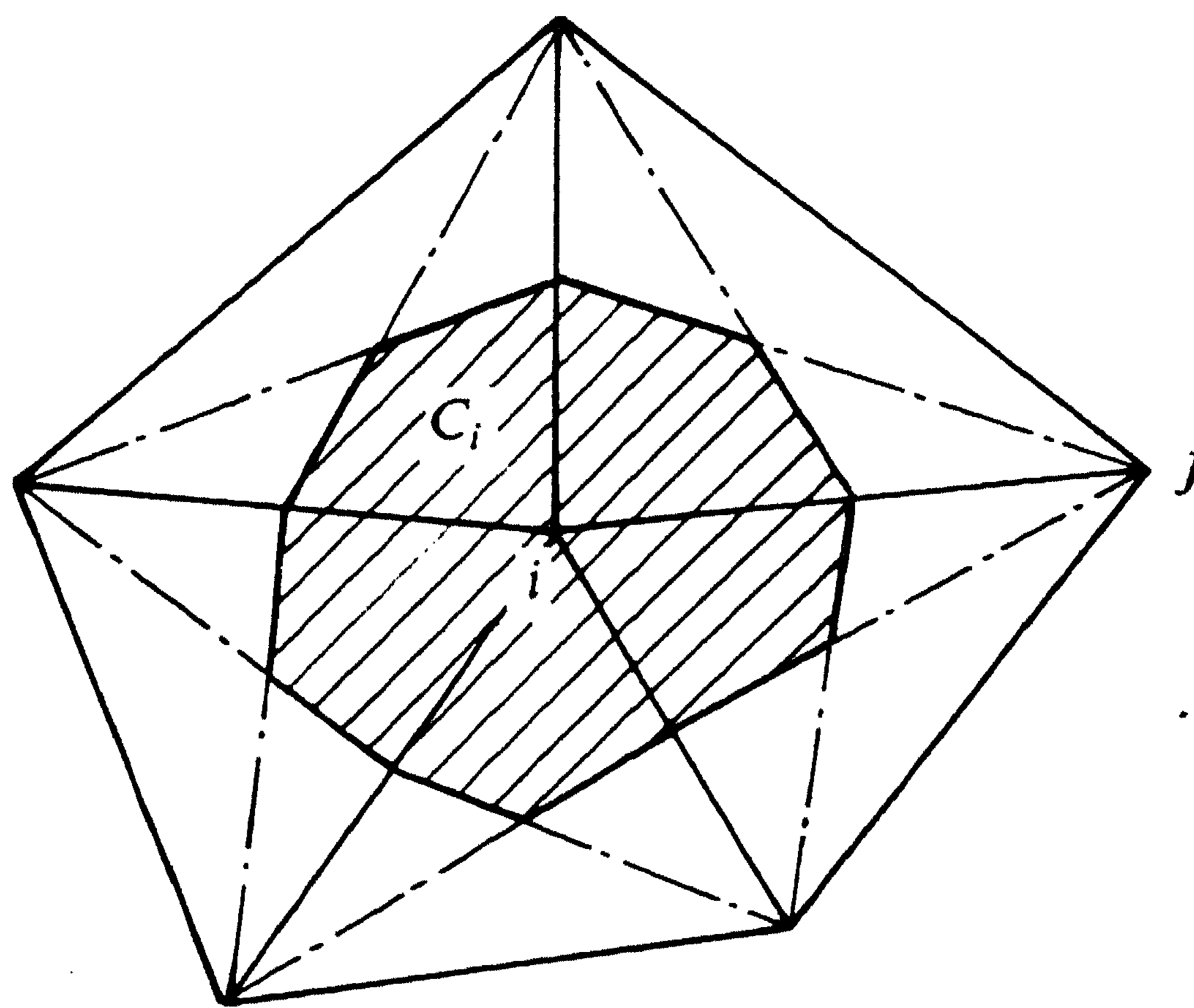
FIGURE 2.1. Finite volume C_i
