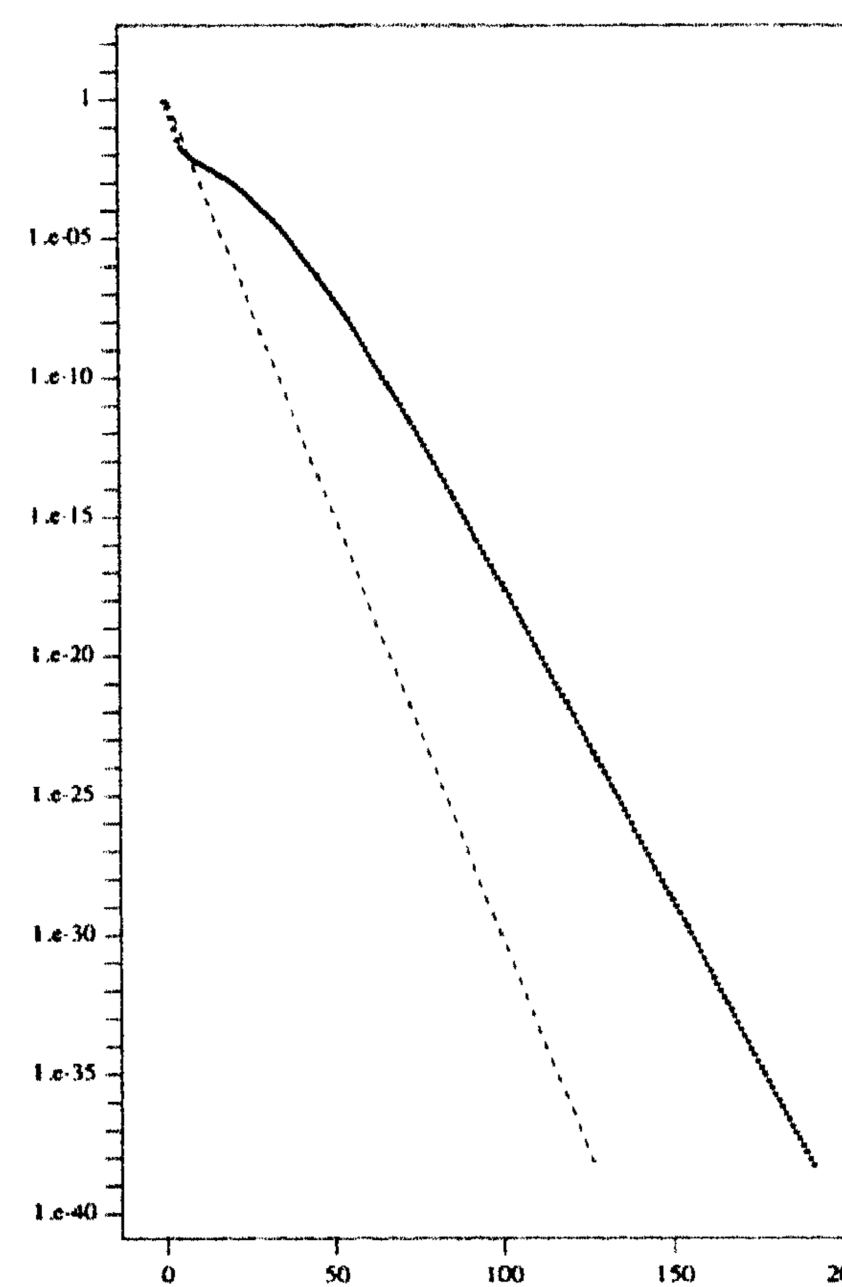
Figure 2.e, 2-dim 40 \times 40 mesh; \kappa = 1/3
