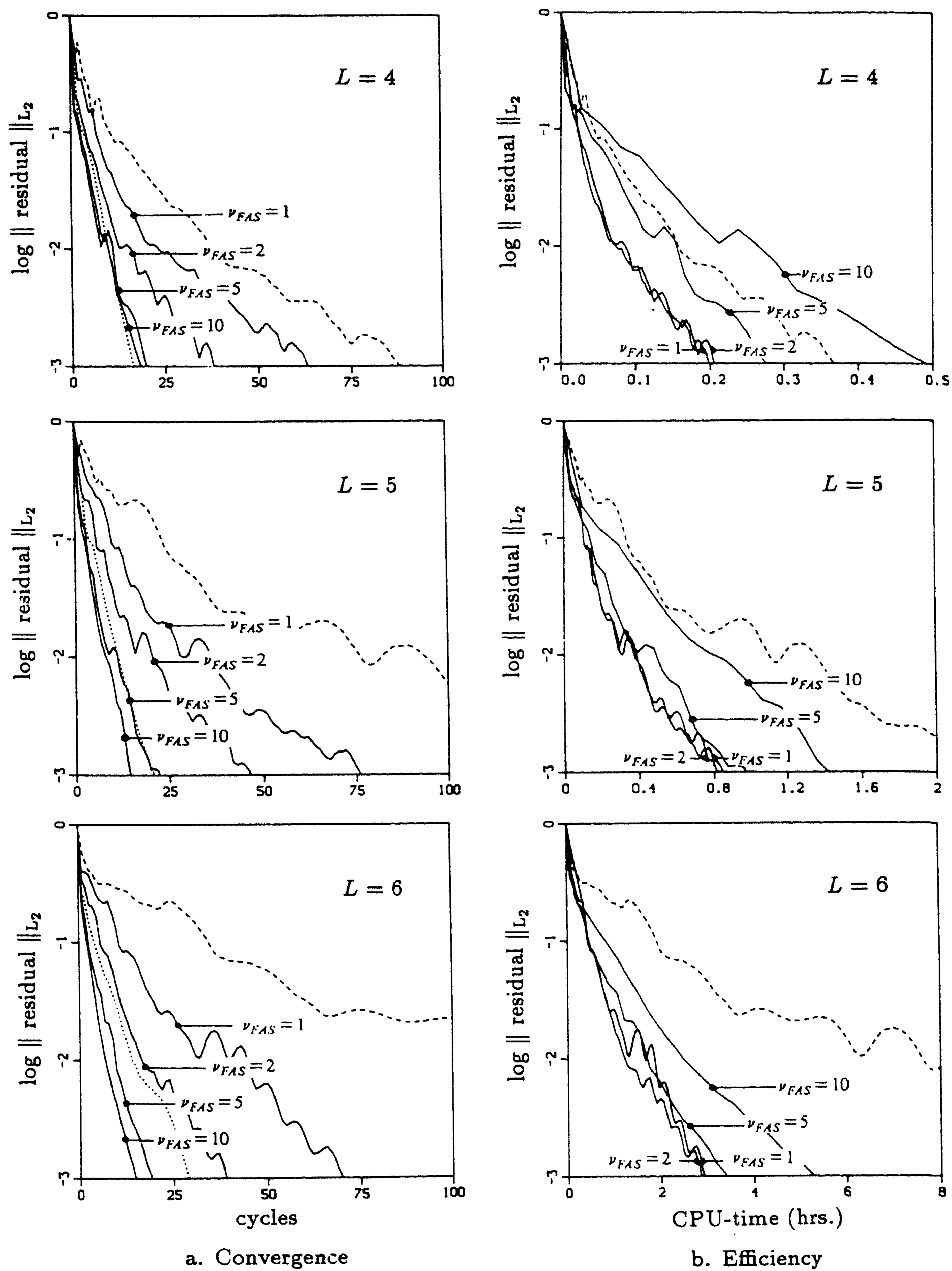
FIGURE 2.3. Convergence and efficiency histories (first-order method: \cdots , existing higher-order method: --- , improved higher-order method: - )
