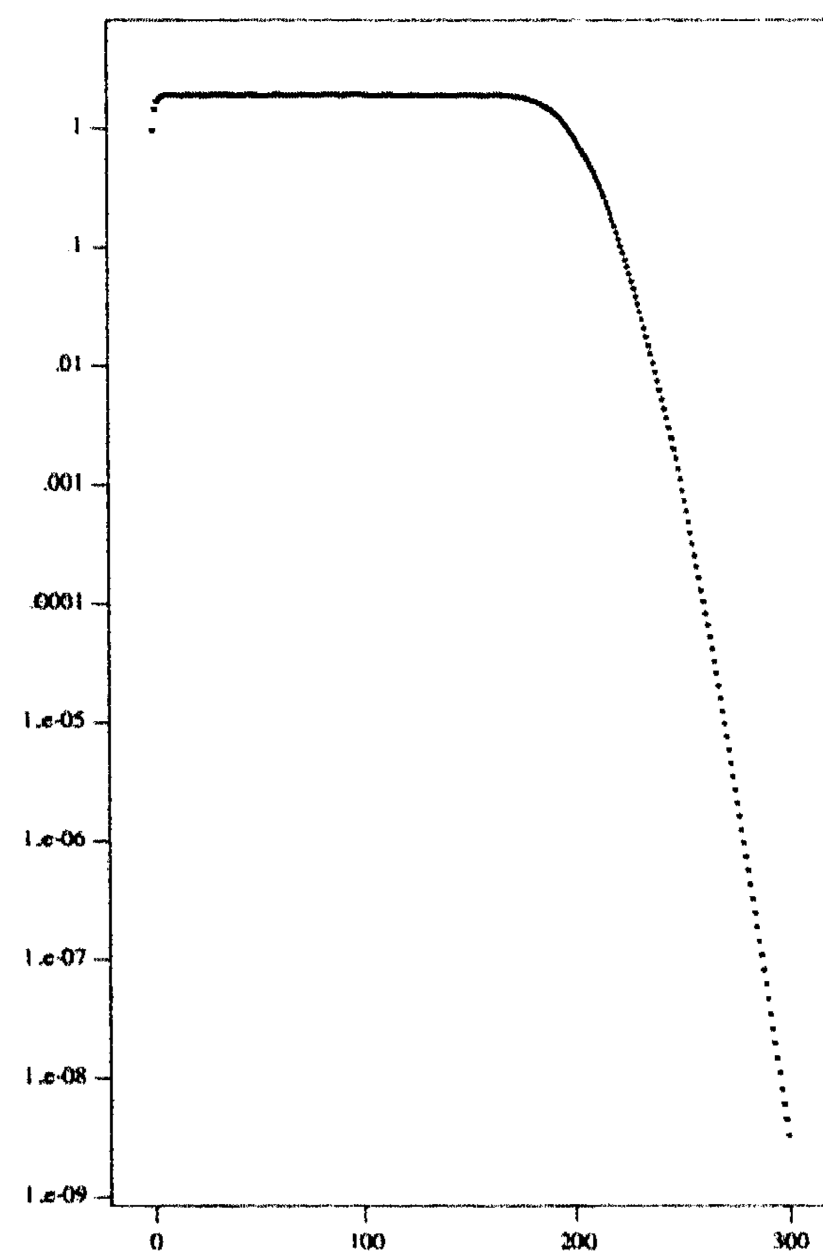
Figure 2.b, 1-dim N = 100; \kappa = 1
