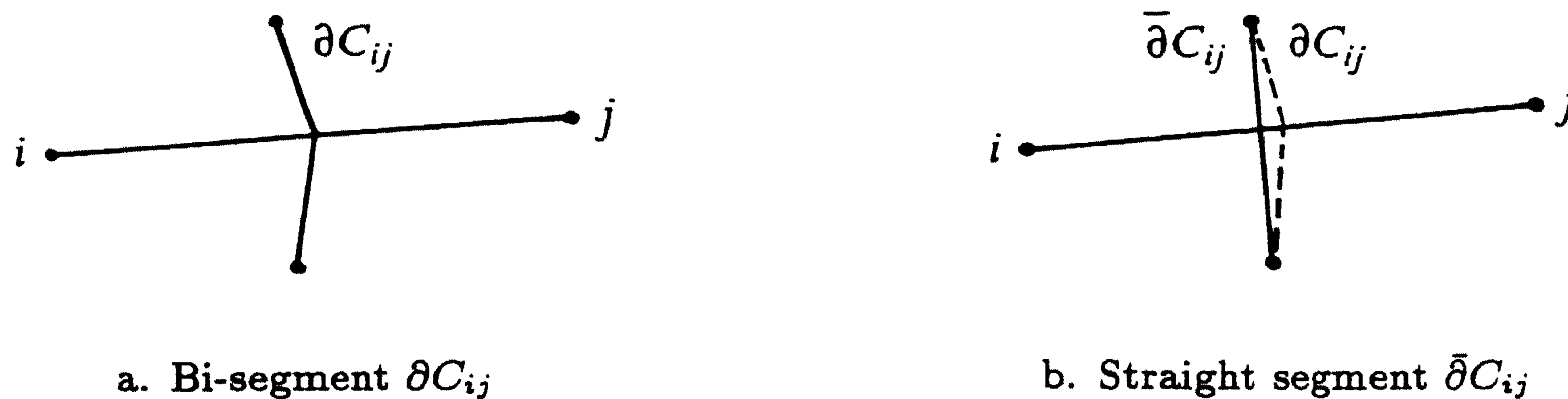
FIGURE 2.2. Segments in between finite volumes C_i and C_j
