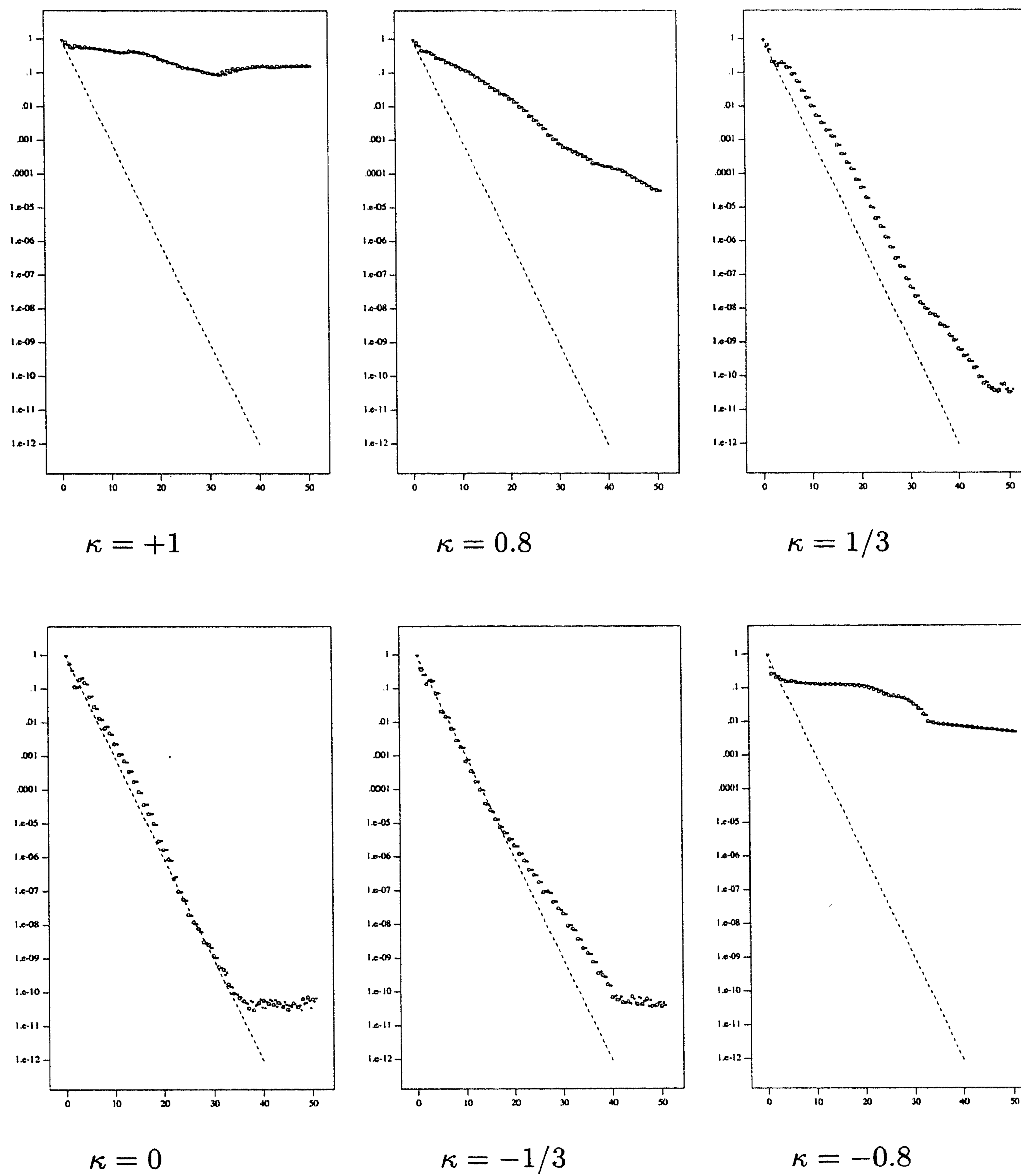
FIGURE 3.3. Subsonic Flow over a NACA0012 Airfoil Convergence of the defect-correction method, on a 20 \times 32 mesh. Mach number at infinity, M_\infty = 0.63 , and the angle of attack \alpha = 2.0^\circ . The dashed line corresponds to a convergence rate 1/2 .
