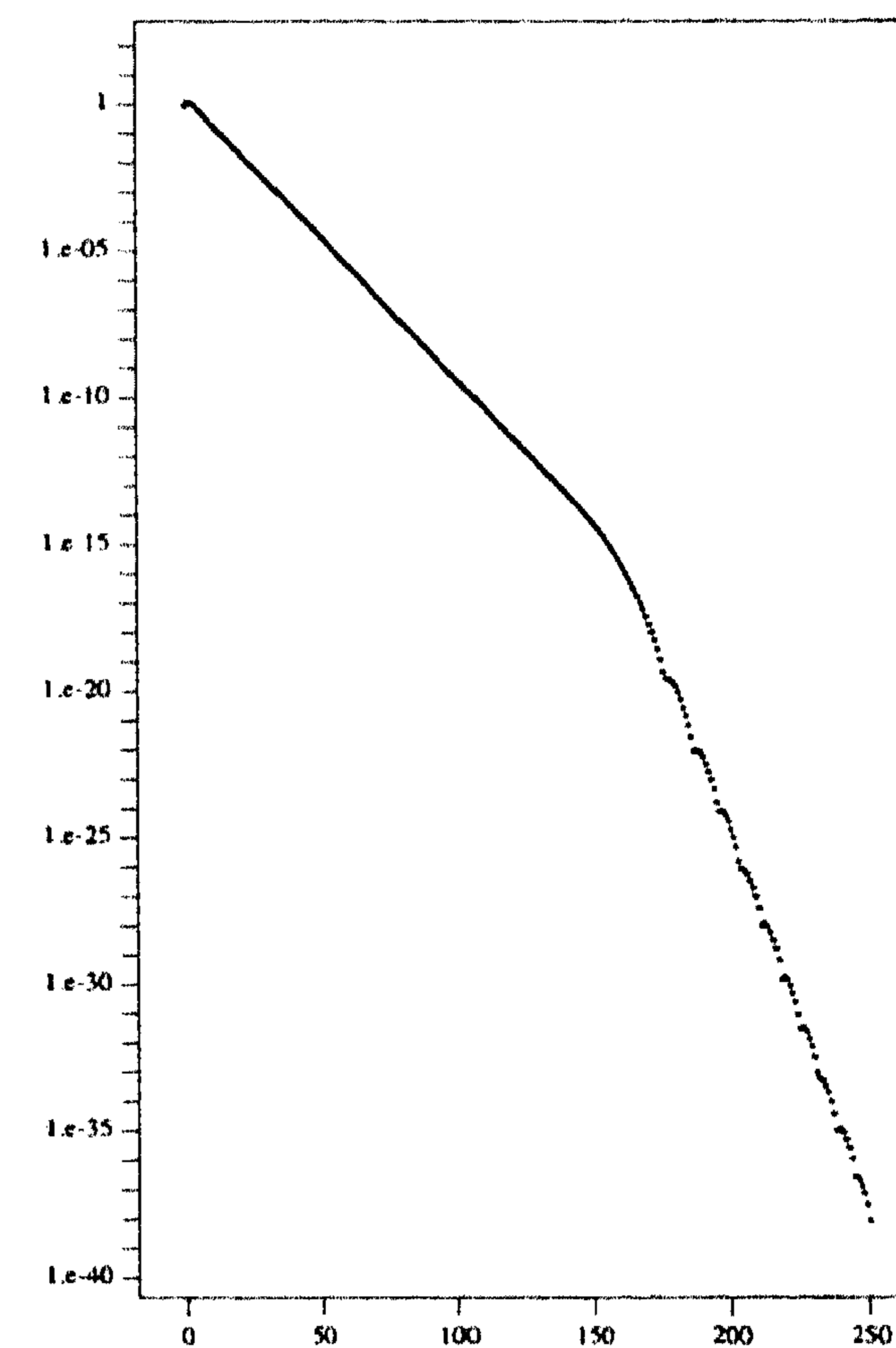
Figure 2.c, 1-dim N = 100; \kappa = 0.8
