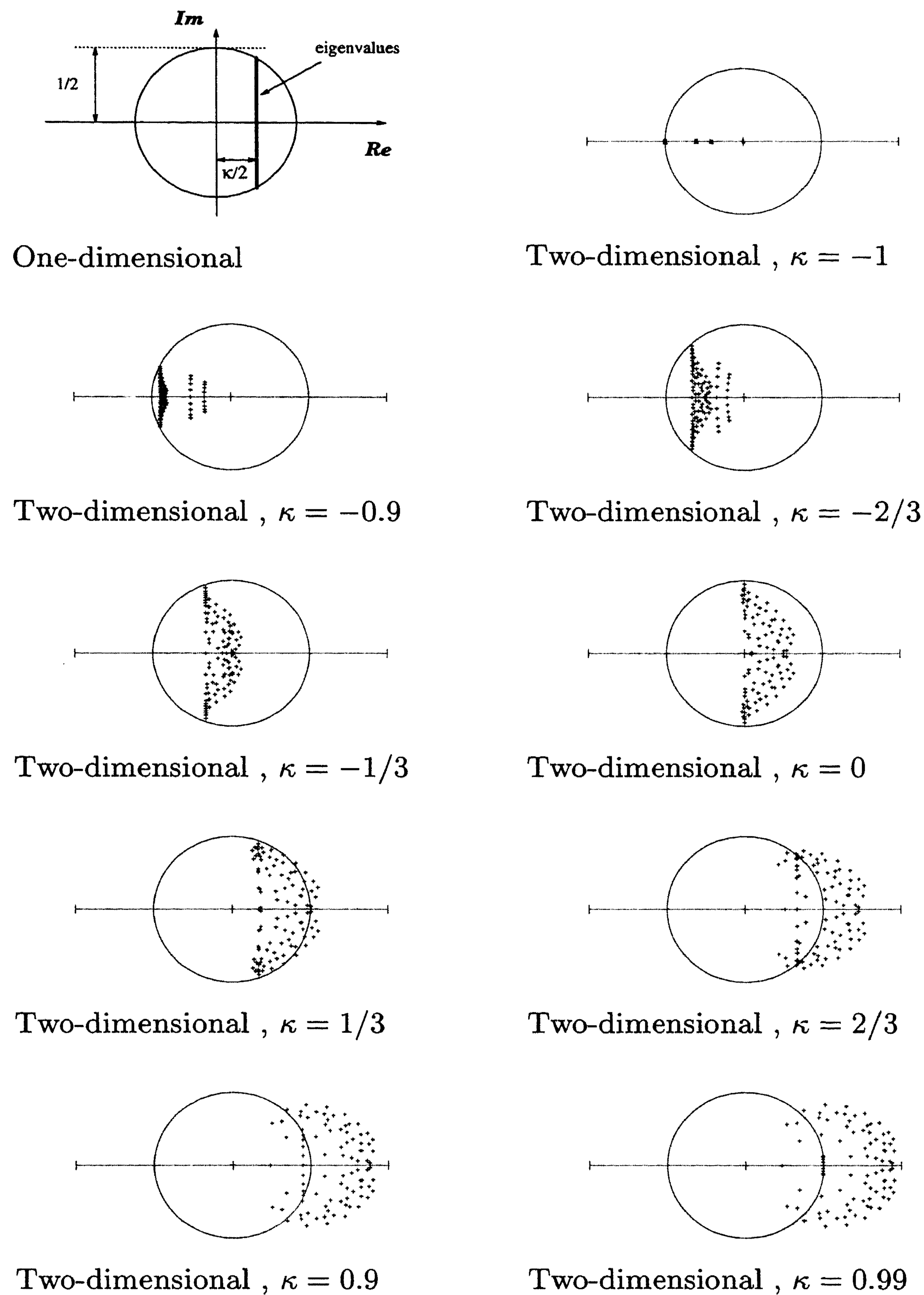
FIGURE 3.1. Location of the eigenvalues of the amplification matrix M_h^\kappa in the complex plane, relatively to the circle of radius 1/2 , for the one and the two-dimensional model problem. Except for the first 1-dim. figure, the mesh is 10 \times 10 and the ratio a/b = 2/3 .
