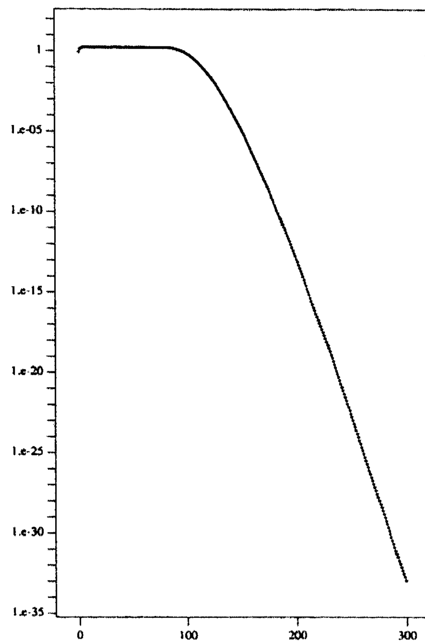
Figure 2.a, 1-dim N = 50; \kappa = 1
