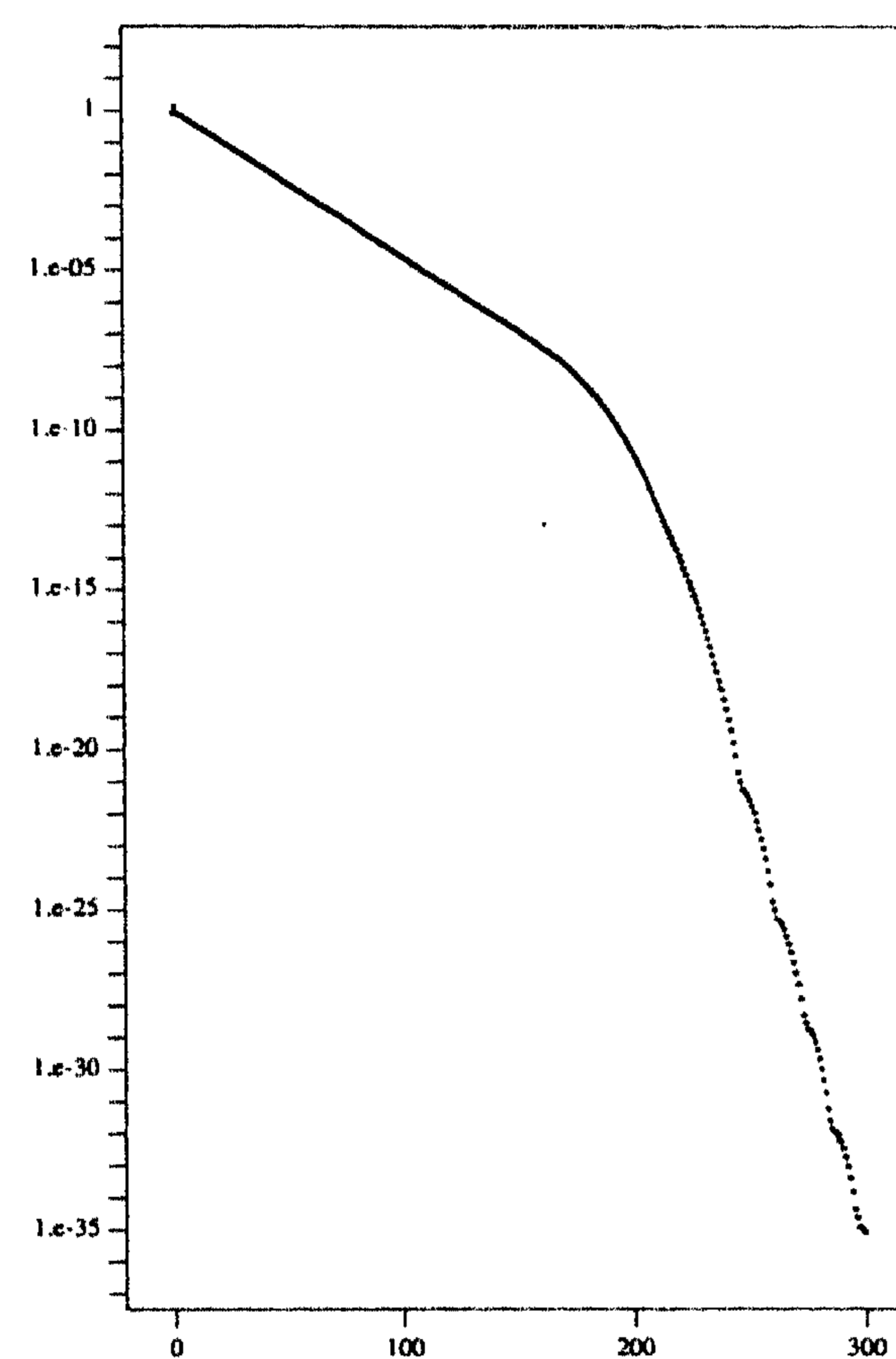
Figure 2.d, 1-dim N = 100; \kappa = -0.9
