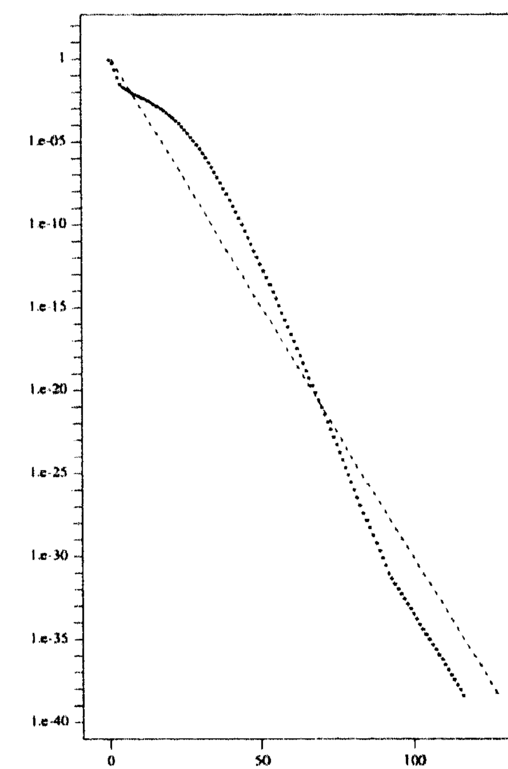
Figure 2.f, 2-dim 40 \times 40 mesh; \kappa = 0
